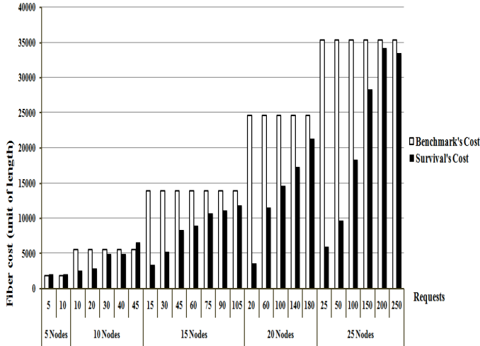
Fig. 3. Fiber cost of network when W = 64 wavelengths
