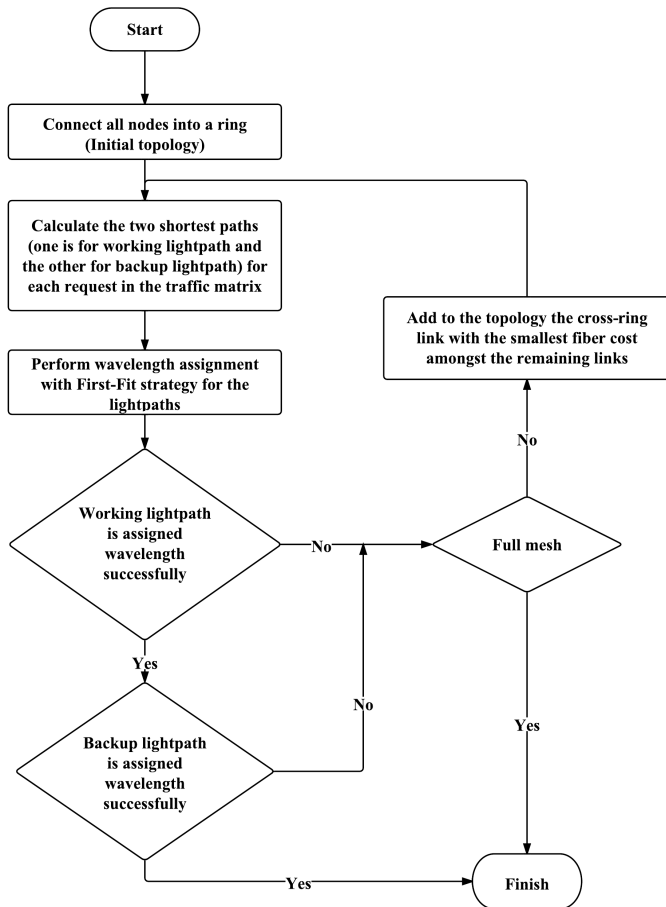
Fig. 1. Flowchart of Survival algorithm
