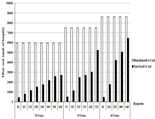
Fig. 4. Fiber cost of network when W = 128 wavelengths
