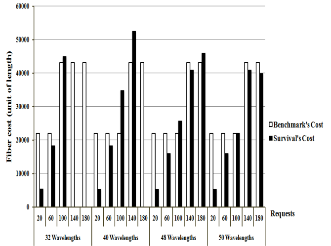
Fig. 5. Fiber costs of Benchmark and Survival when the number of wavelengths per link increases.
